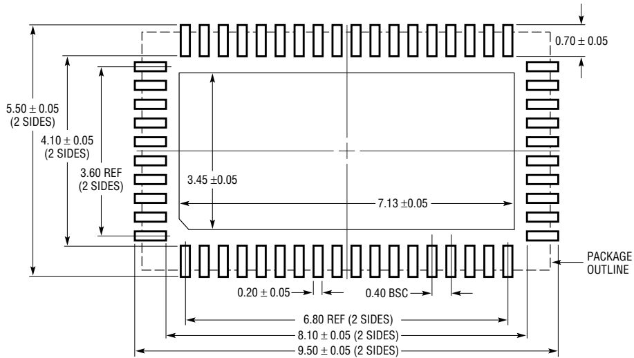
UHH Package 56-Lead Plastic QFN (5mm × 9mm) (Reference LTC DWG # 05-08-1727 Rev A)
