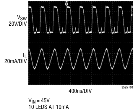
Figure 1. Switching Waveforms
